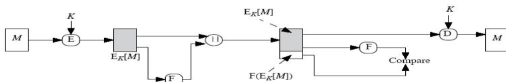
(b) External error control
