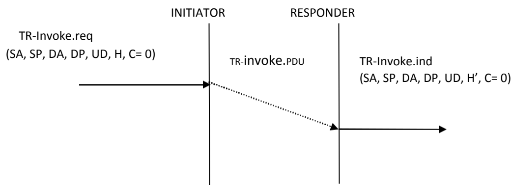
Fig 11.5 Class 0 Basic Transaction
