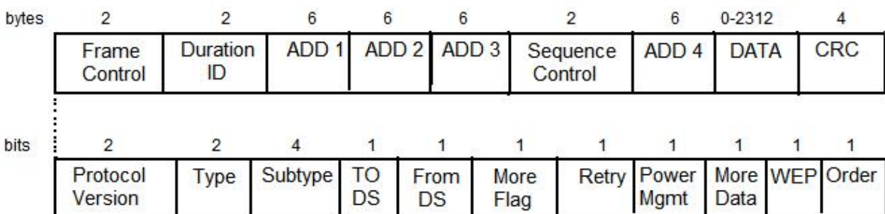
Fig 9.6 IEEE 802.11 MAC packet structure
