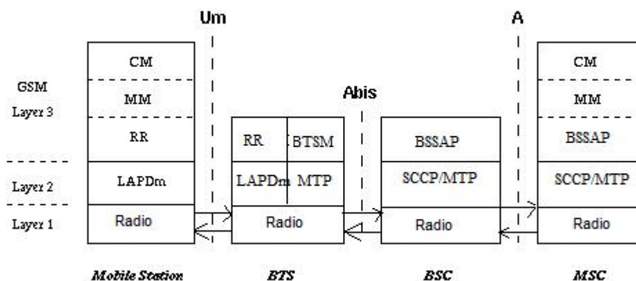
Fig 6.4 Network Signaling
