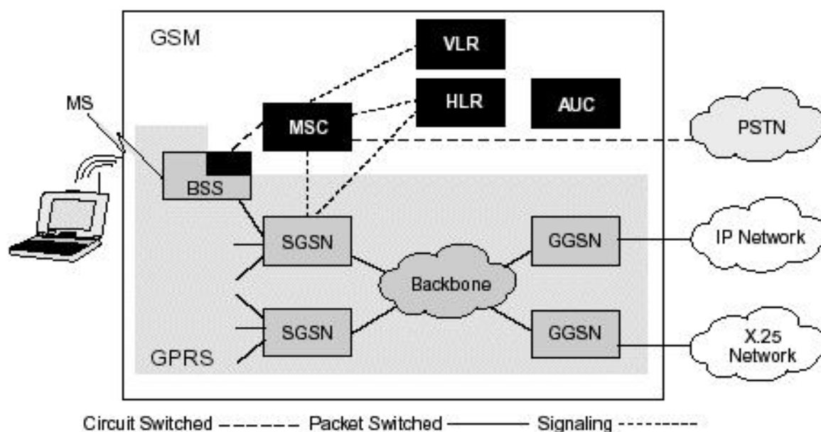
Fig 7.1 GPRS Architecture
