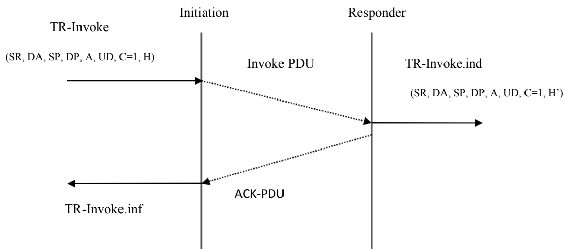
Fig 11.6 Class 1 Basic Transaction
