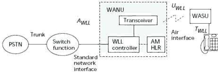
Fig 12.2 WLL Architecture
